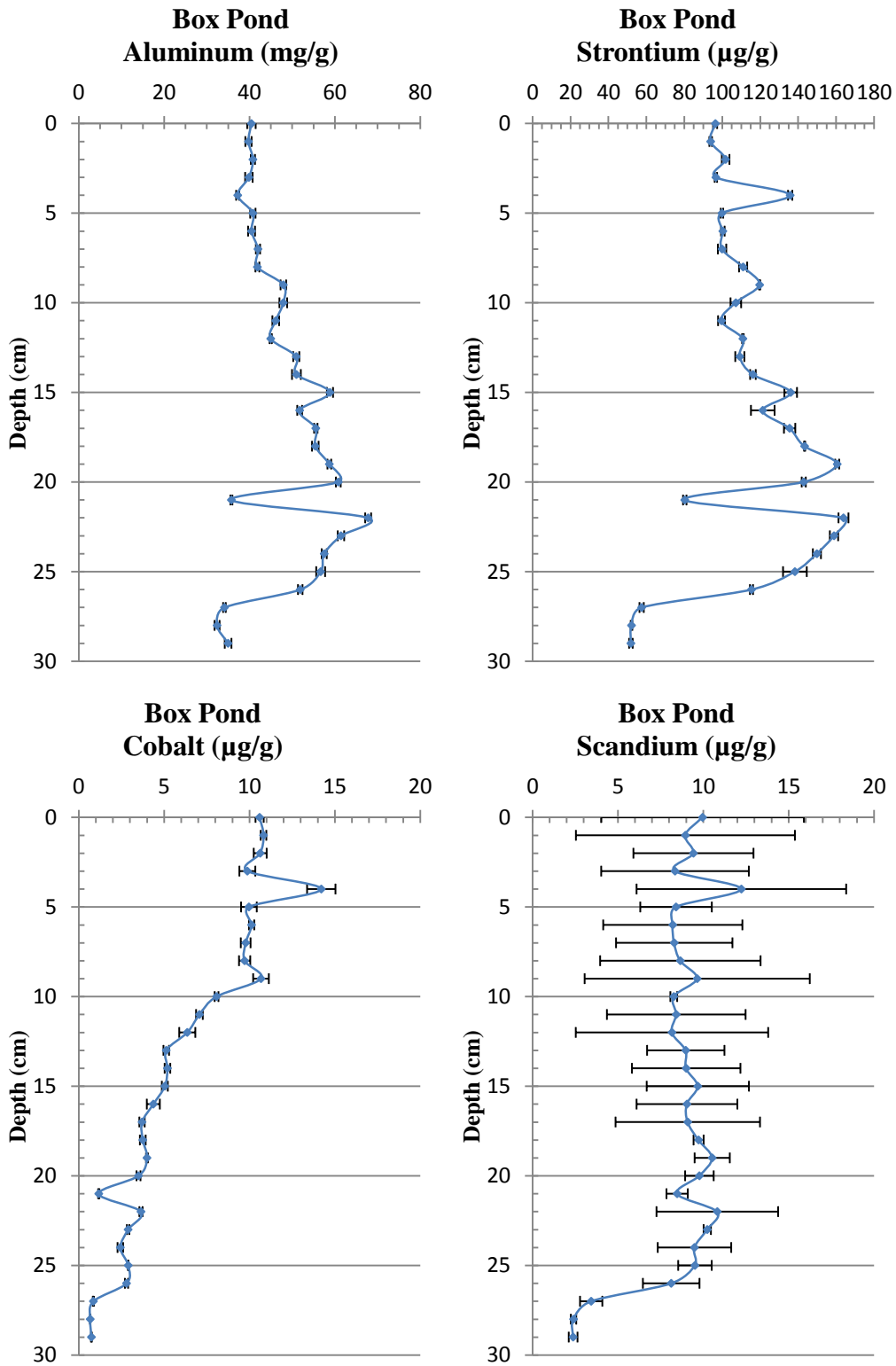
Figure II.5. Box Pond sediment core crustal indicator metals.
