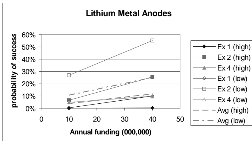
Figure 1: Probabilities of Success for Batteries with Lithium Metal Anodes
